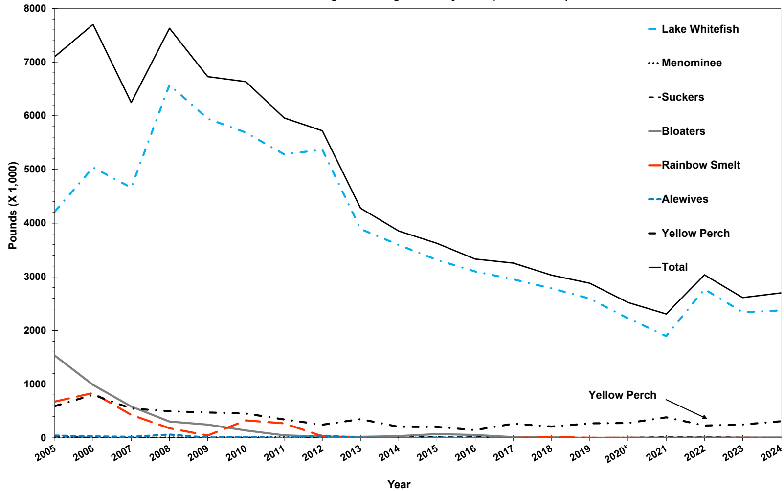
Figure 5b. This chart highlights annual harvest of select species from Lake Michigan during the last 20 years (2005-2024) and is a subset of the data provided in Fig 5a; note associated change in scale.
